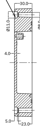
SECTION B-B
